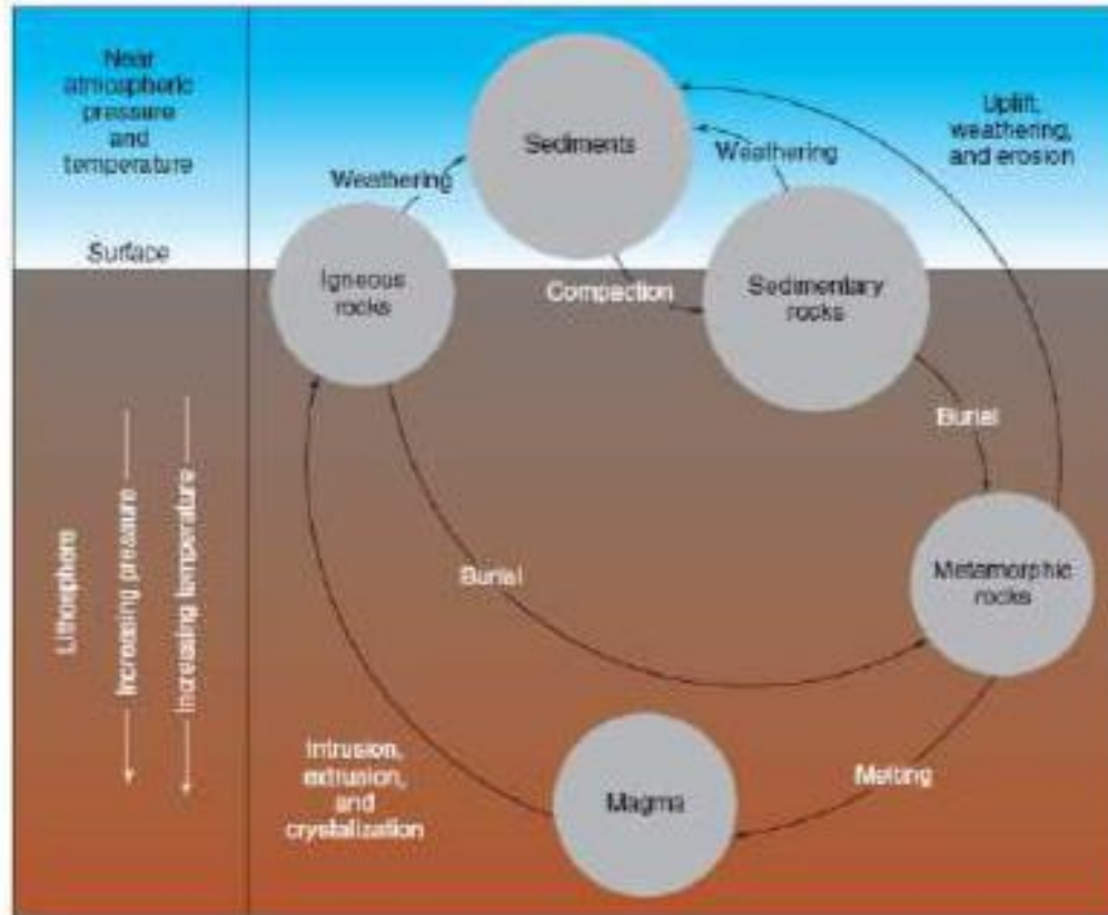
Fig.4 Rock Cycle
