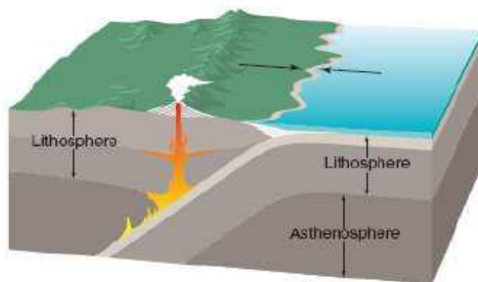
FIG: 6 A convergent plate boundary where an oceanic plate subducts under a continental plate
